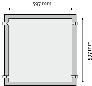
View D500
